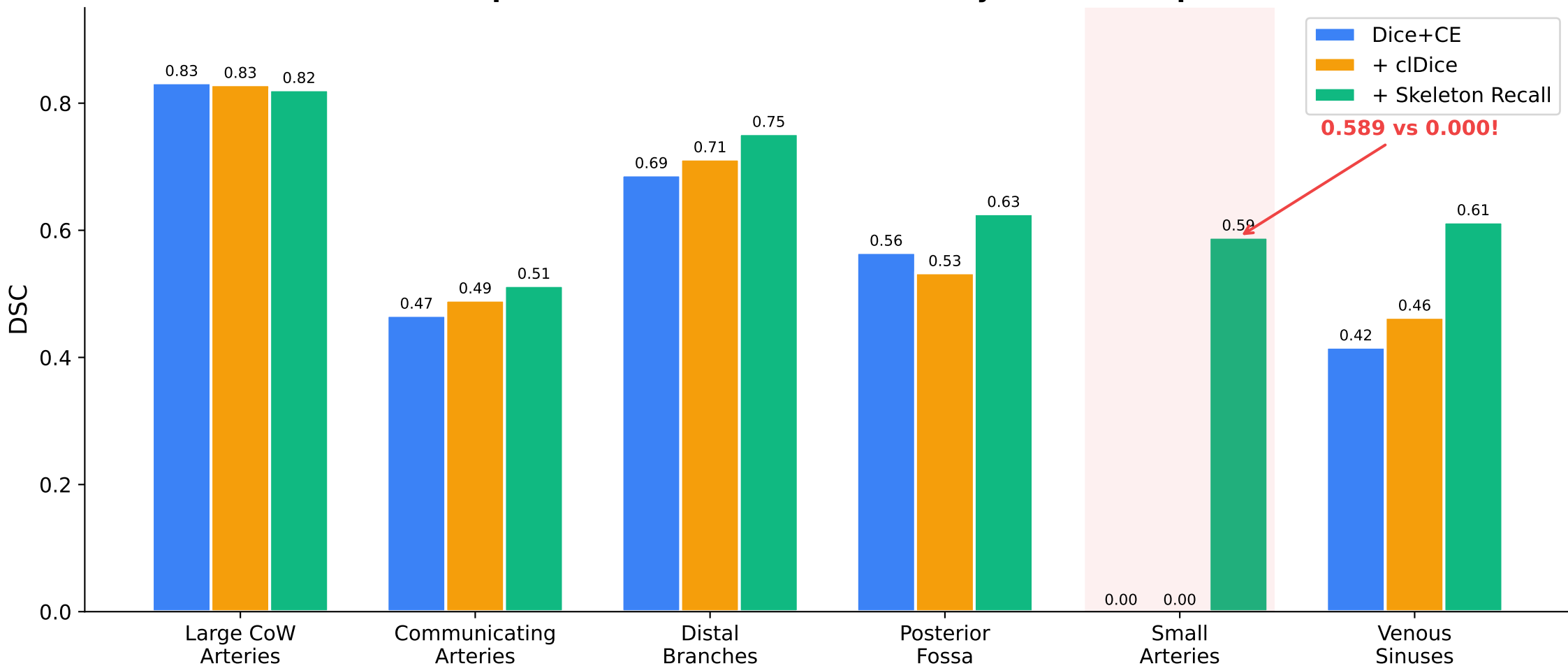
TopBrain Fine-Tuned Models: DSC by Vessel Group
